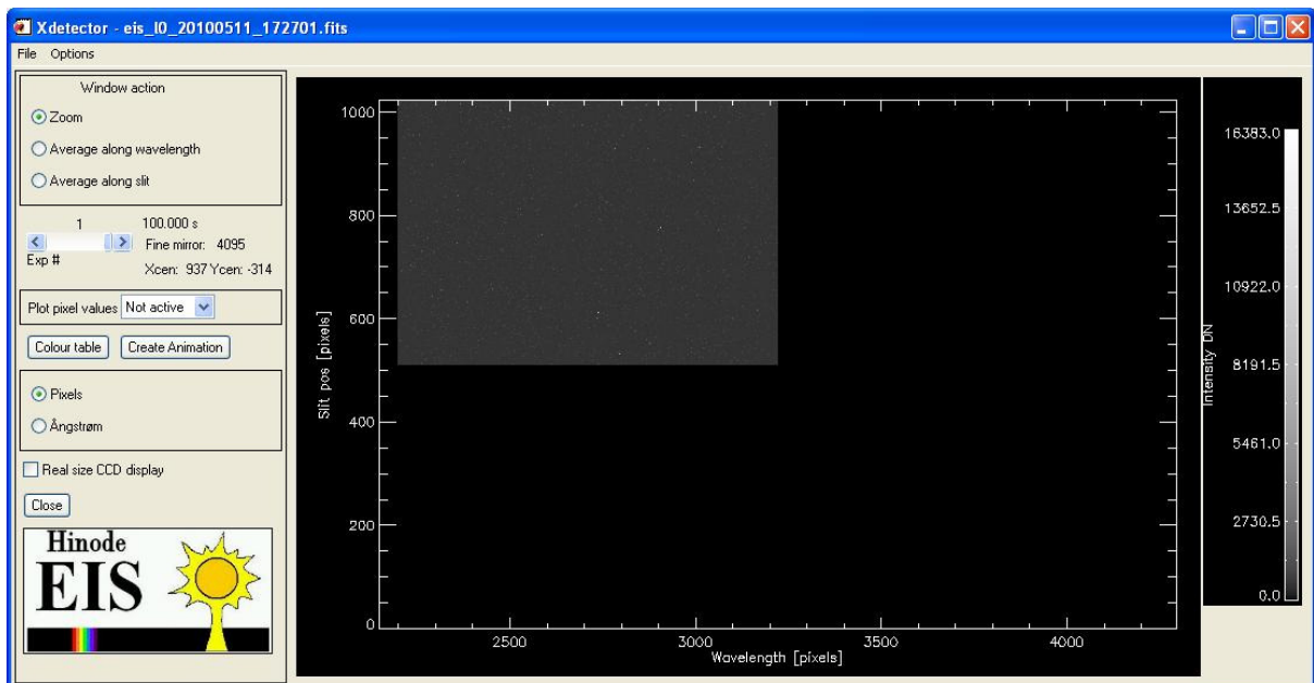
Long wavelength CCD, 2 nd exposure, right side of CCD missing, left side data ok
