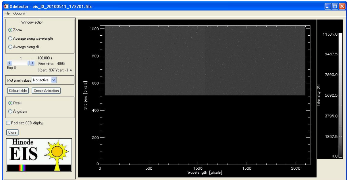
Short wavelength CCD, 2 nd exposure complete (data ok)
