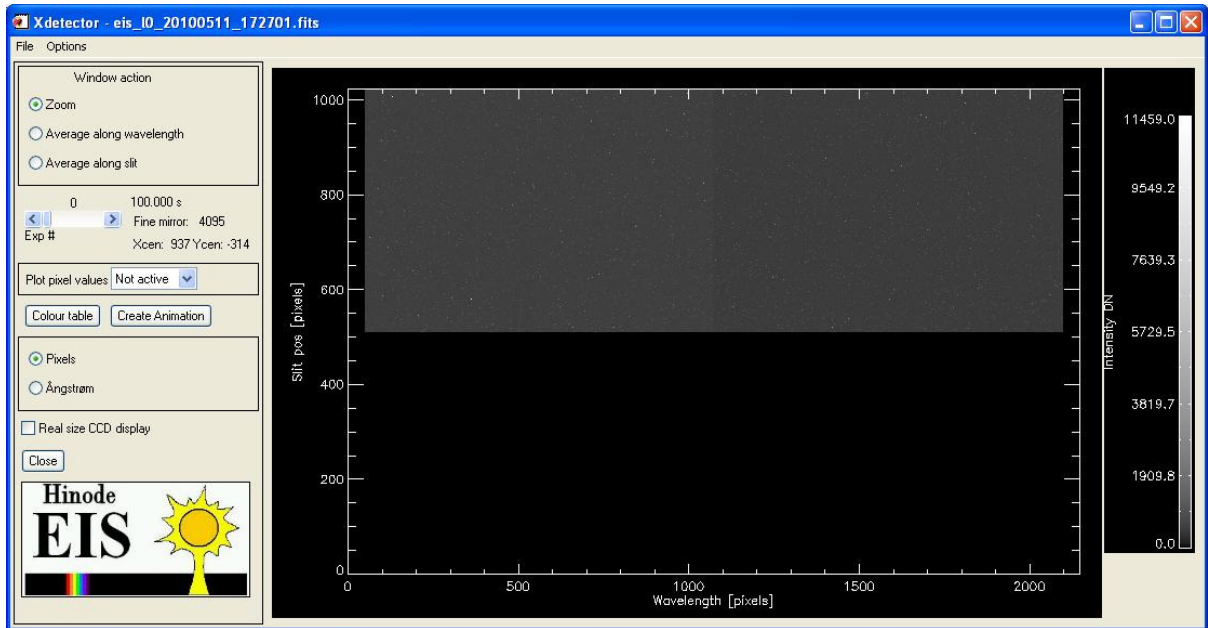
Short wavelength CCD, 1 st exposure complete (data ok)
