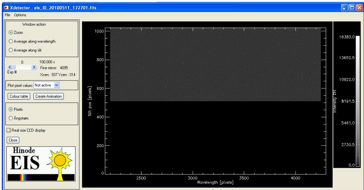
Long wavelength CCD, 1 st exposure complete (data ok)
