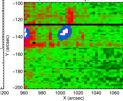
c; EIS He II intensity, T=15:42
