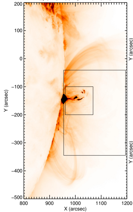
a; SDO 193 Å, T=15:49:28
