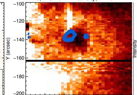
c; EIS He II intensity, T=15:42
