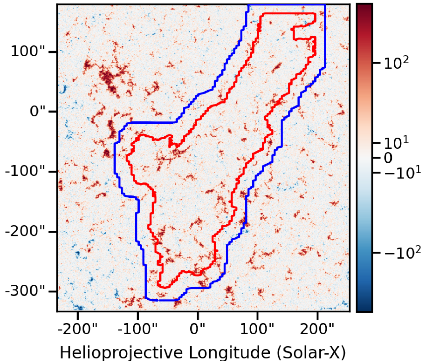
HMI Magnetogram 2016-03-25T11:10:15.200
